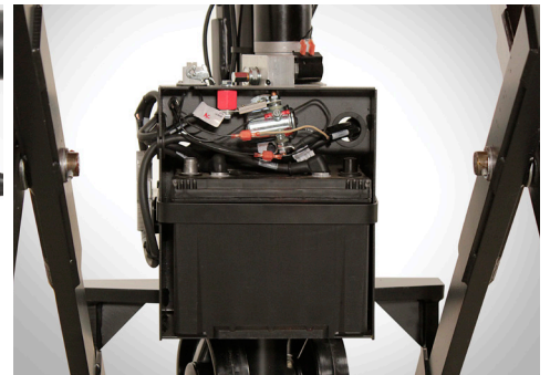
Electric lift by 12V DC hydraulic power pack (Electric model)
